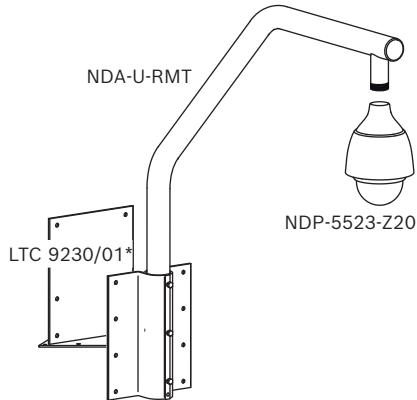
Fig. 4: Roof mount (IP66) *Optional for flat roof mount
